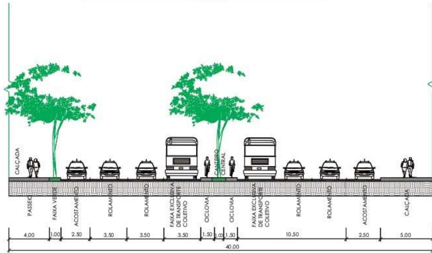
VIA ARTERIAL I
