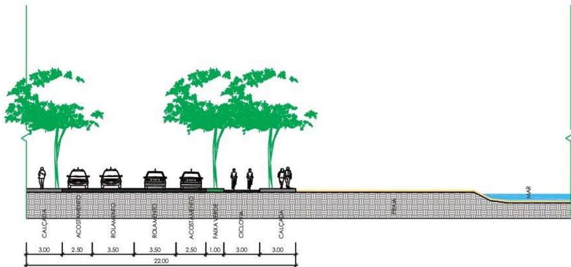
VIA ARTERIAL III
