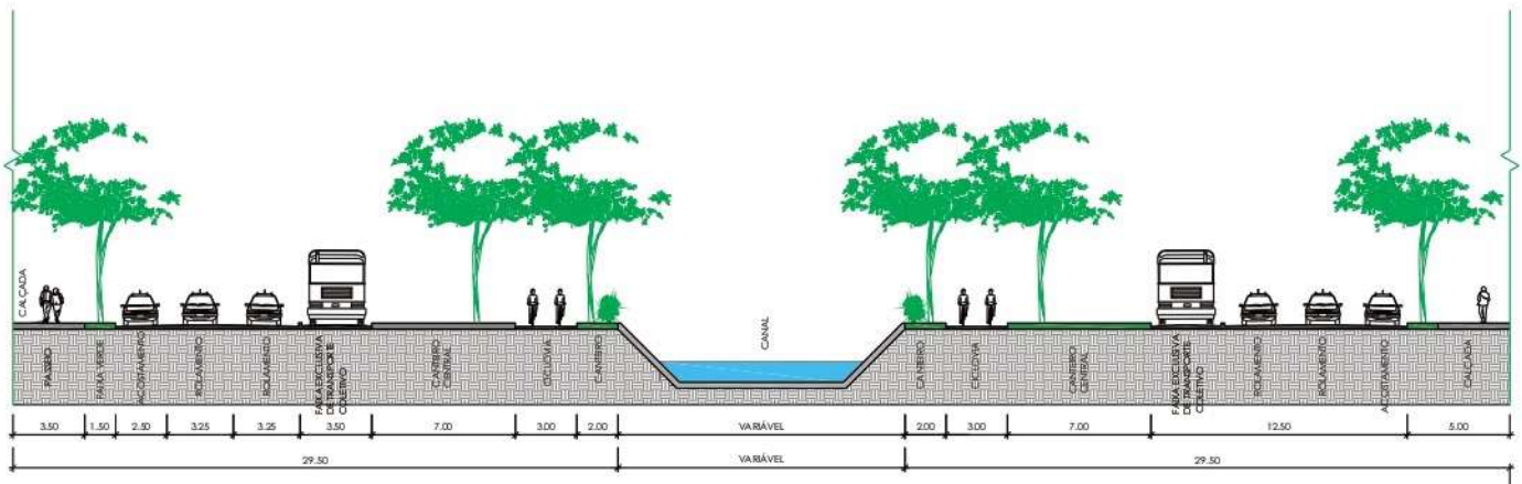
VIA ARTERIAL II
